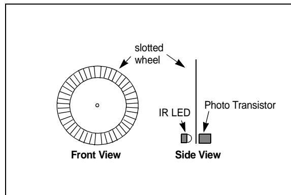
FIGURE 9: OPTICAL ENCODER
