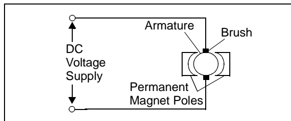
FIGURE 2: PERMANENT MAGNET DC MOTORS
